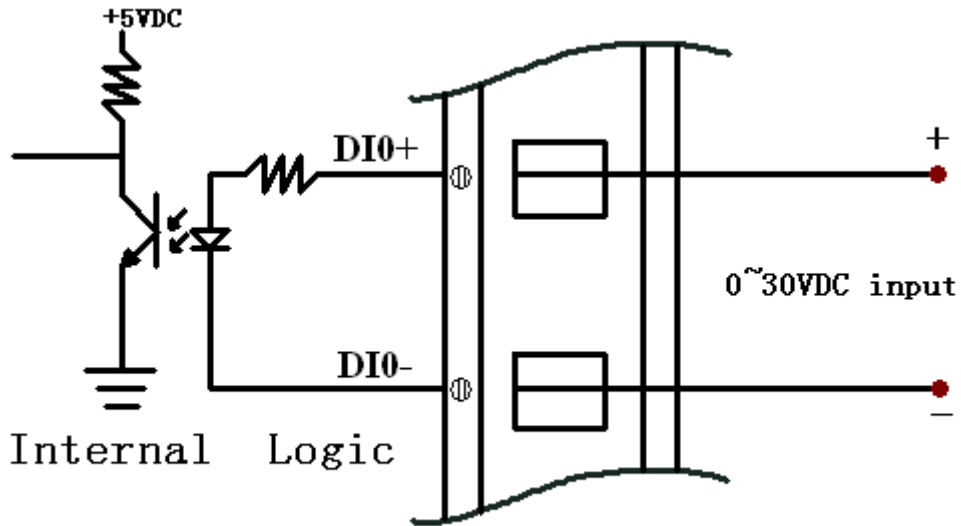
External Wiring (external connect with 0 ~ 30V)
